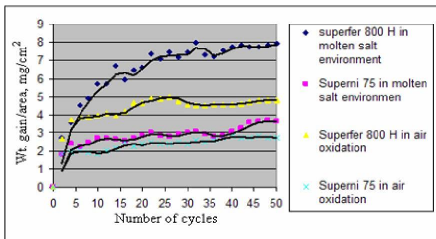
Figure 1. Weight gain/area versus number of cycles plot for the Superni 75 and Superfer 800H Super alloys subjected to air and molten salt ( \text{Na}_2\text{SO}_4 -25% NaCl) environments for 50 cycles at 800^\circ\text{C} .
