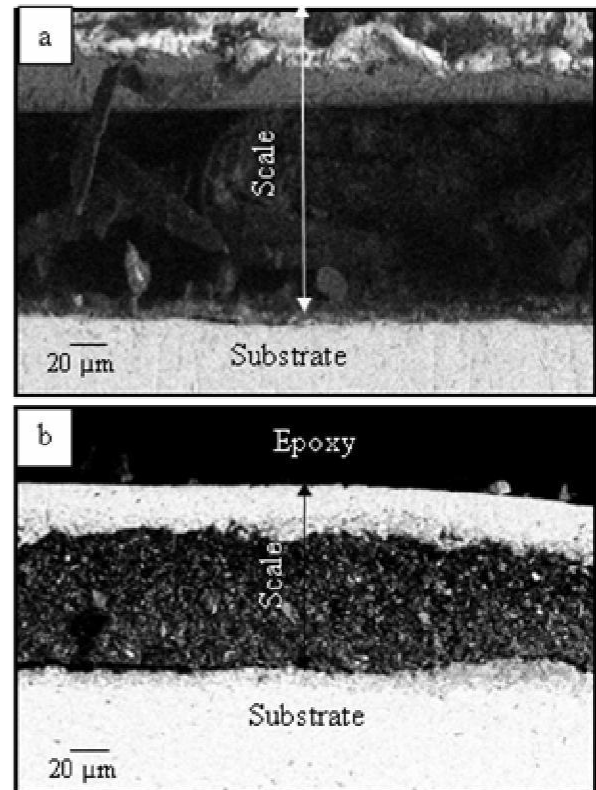
Figure 5. BSE images across the cross-section of hot corroded superalloys after subjecting to molten salt ( \text{Na}_2\text{SO}_4 + 25\%\text{NaCl} ) environment at 800^\circ\text{C} for 50 cycles: (a) Superfer 800H (b) Superni 75.
