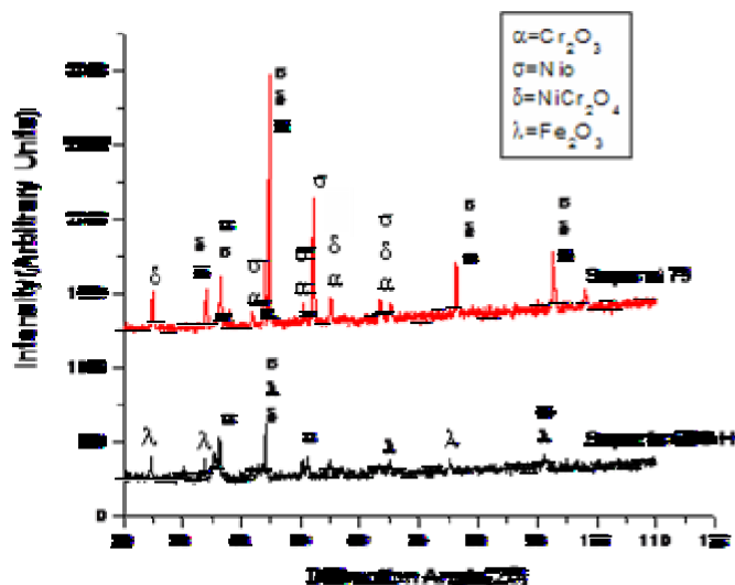
Figure 6. XRD of corroded superalloys after exposure to air oxidation for 50 cycles at 800°C.
