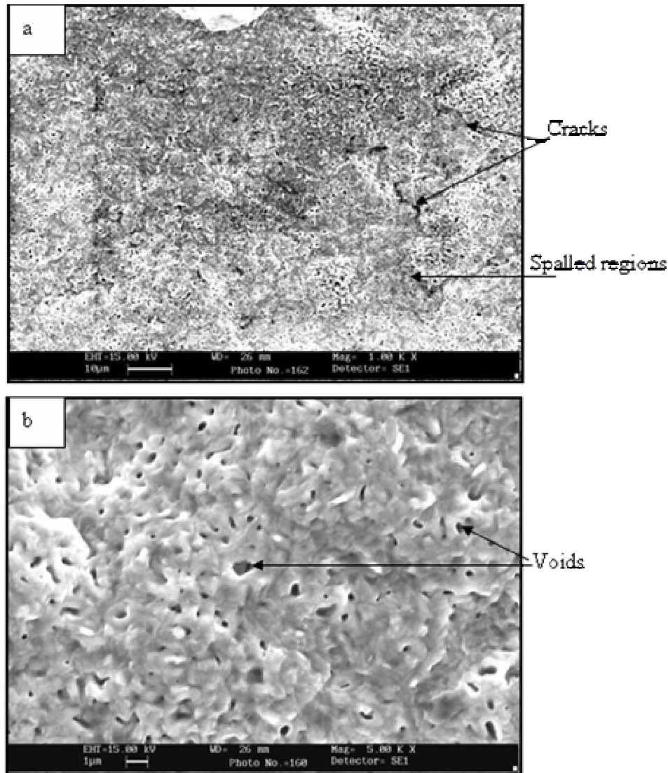
Figure 3. SEM of Superfer 800H after hot corrosion in molten salt environment of \text{Na}_2\text{SO}_4+25\%\text{NaCl} for 50 cycles at 800^\circ\text{C} .
