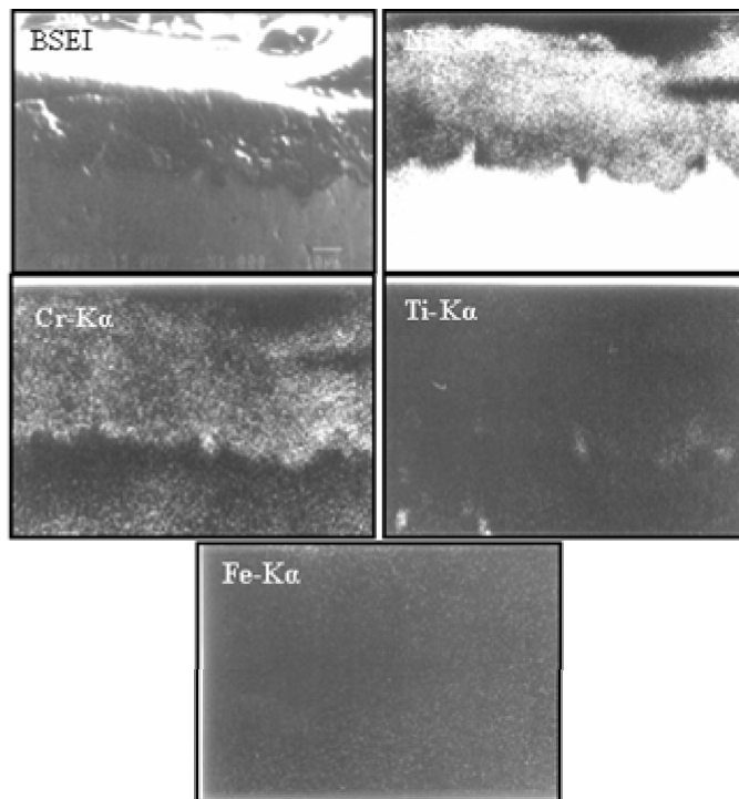
Figure 8. Composition image (BSEI) and X-ray mappings of the cross-section of the Superalloy 75 subjected to hot corrosion at 800°C in Na 2 SO 4 -25%NaCl environment for 50 cycles.
