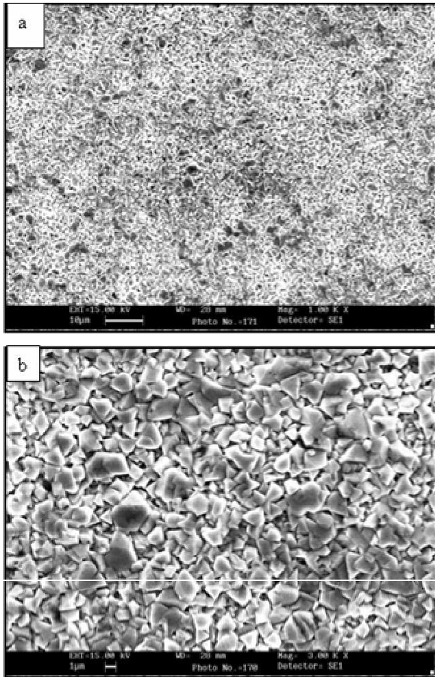
Figure 4. SEM of Superni 75 after hot corrosion in molten salt environment of \text{Na}_2\text{SO}_4 + 25\%\text{NaCl} for 50 cycles at 800^\circ\text{C} .
