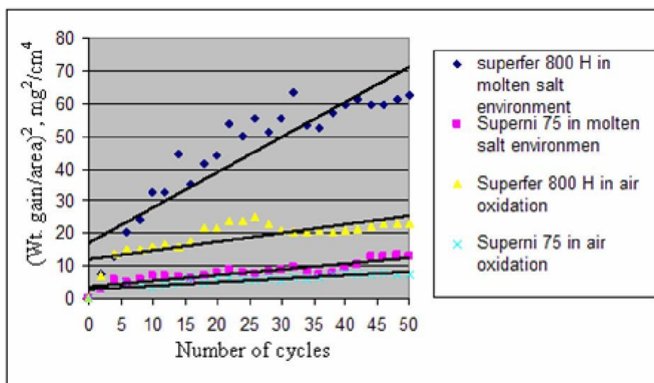
Figure 2. (\text{Weight gain/area})^2 versus number of cycles plot for the Superni 75 and Superfer 800H superalloys subjected to air and molten salt ( \text{Na}_2\text{SO}_4 -25%NaCl) environments for 50 cycles at 800^\circ\text{C} .
