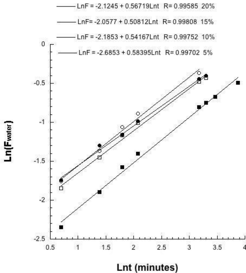
Figure A. Plot equation 12 for determining if the diffusion follows the law of Fick for hidrogeles place in water.
