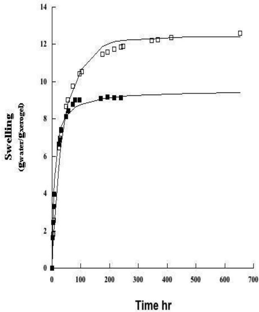
Figure 1. Comparison between the experimental data and the model of the swelling kinetics, for polyacrylamide hydrogel 20% in water (■) in saline at 100% (□).
