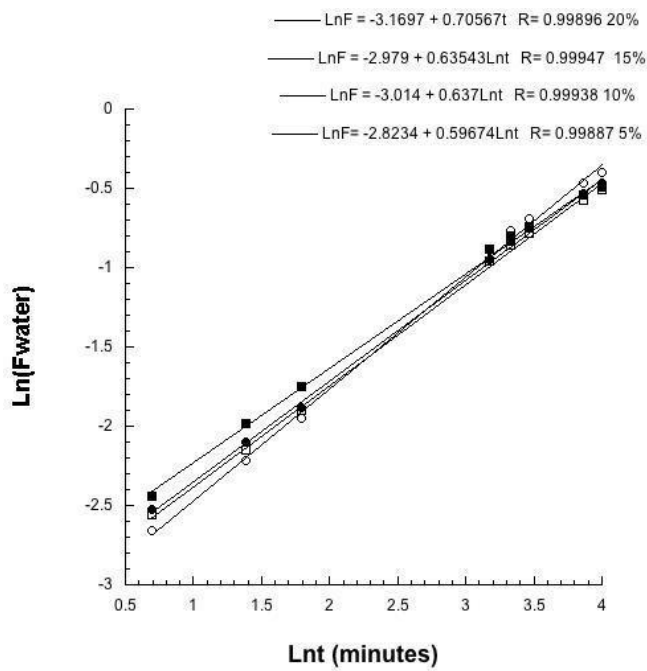
Figure B. Plot equation 12 for determining if the diffusion follows the law of Fick. For hidrogeles place in solution of 100% saturation.
