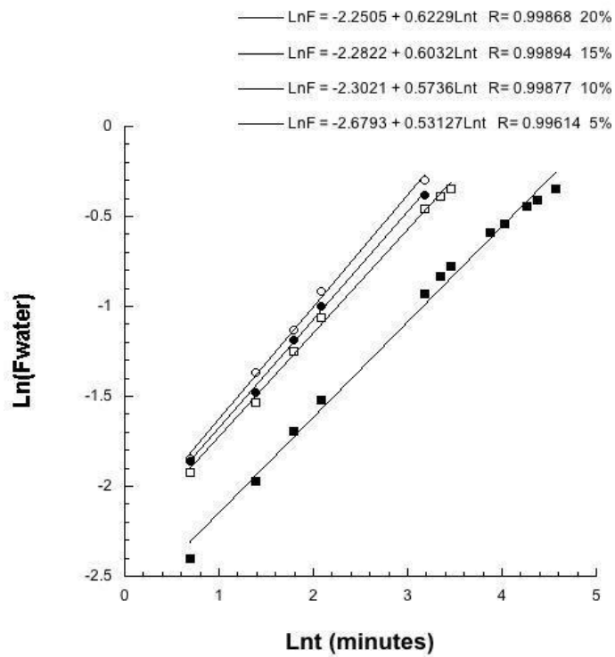
Figure C. Plot equation 12 for determining if the diffusion follows the law of Fick for hidrogeles place to solution of 100% saturation.
