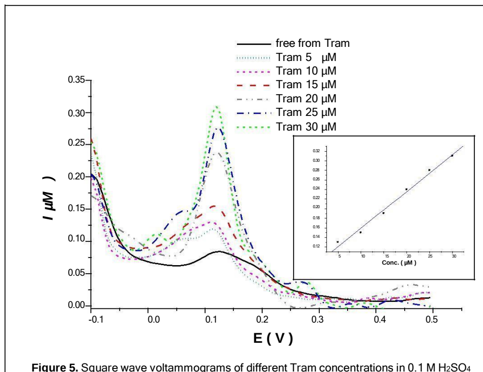
Figure 5. Square wave voltammograms of different Tram concentrations in 0.1 M \text{H}_2\text{SO}_4 aqueous solution and blank solution (Tram free solution) at PAMDAN/Pt modified electrode at scan rate 5 mV/s. Inset: Plot of peak currents as a function of Tram concentration.
