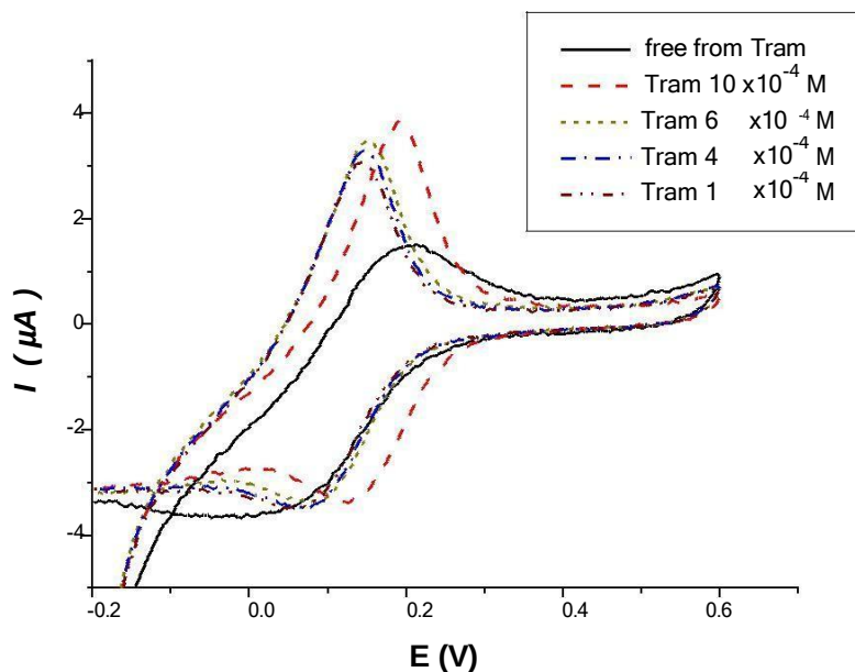
Figure 4. Cyclic voltammograms of different Tram concentrations in 0.1 M \text{H}_2\text{SO}_4 aqueous solution and blank solution (Tram free solution) at PAMDAN/Pt modified electrode at scan rate of 0.1 V/s.
