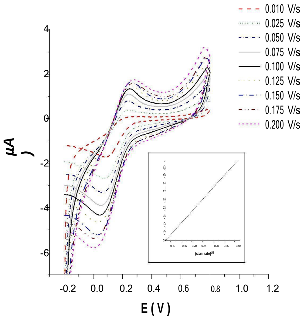
Figure 3. Cyclic voltammograms of 1 \times 10^{-4} M of Tram in 0.1 M \text{H}_2\text{SO}_4 at PAMDAN/Pt modified electrode at different scan rates. The inner diagram represents the plot of I_{pa} vs. square root of scan rate ( u^{1/2} ) for Tram at PAMDAN/Pt modified electrode. The regression equation is I_{pa} = (-0.49) + (5.82) u^{1/2} .
