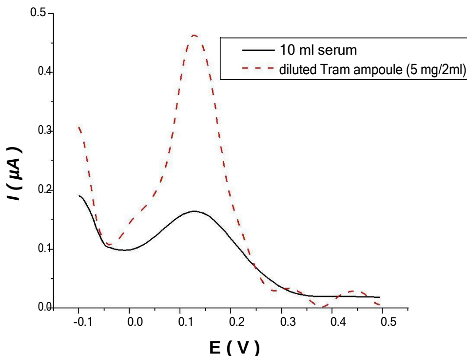
Figure 6. Square wave voltammograms of 5 mg/2 ml Tram in its pharmaceutical forms (Tram ampoule) and the human blood serum sample in 0.1 M H 2 SO 4 at PAMDAN/Pt at a scan rate of 5 mV/s.
