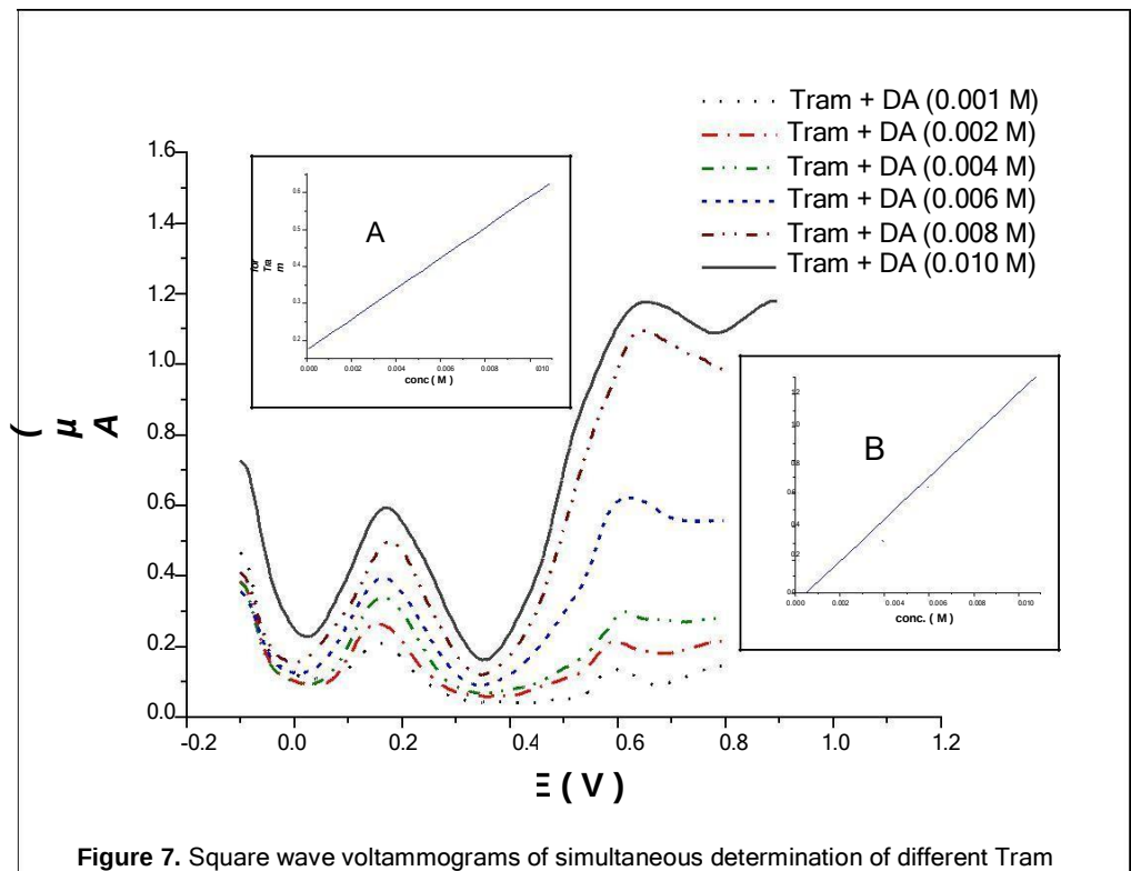
Figure 7. Square wave voltammograms of simultaneous determination of different Tram and DA concentrations at PAMDAN/Pt modified electrode at scan rate of 5 mV/s. Insets: (A) Plot of peak currents as a function of Tram concentration. (B) Plot of peak currents as a function of DA concentration. Table 5. The characteristics of the calibration curves of Tram individually and in mixture with DA in solution at P/PAMADAN.
