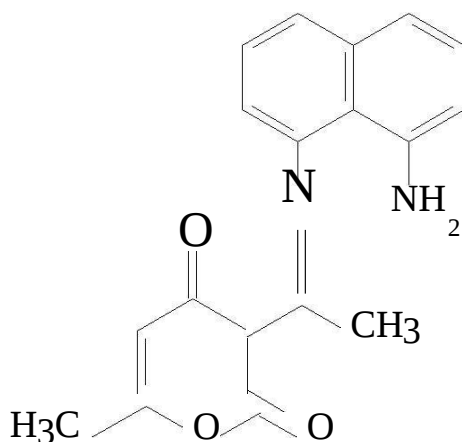
Figure 1. 8-(3-acetylimino-6-methyl-2,4-dioxopyran)-1-aminonaphthalene (AMDAN).
