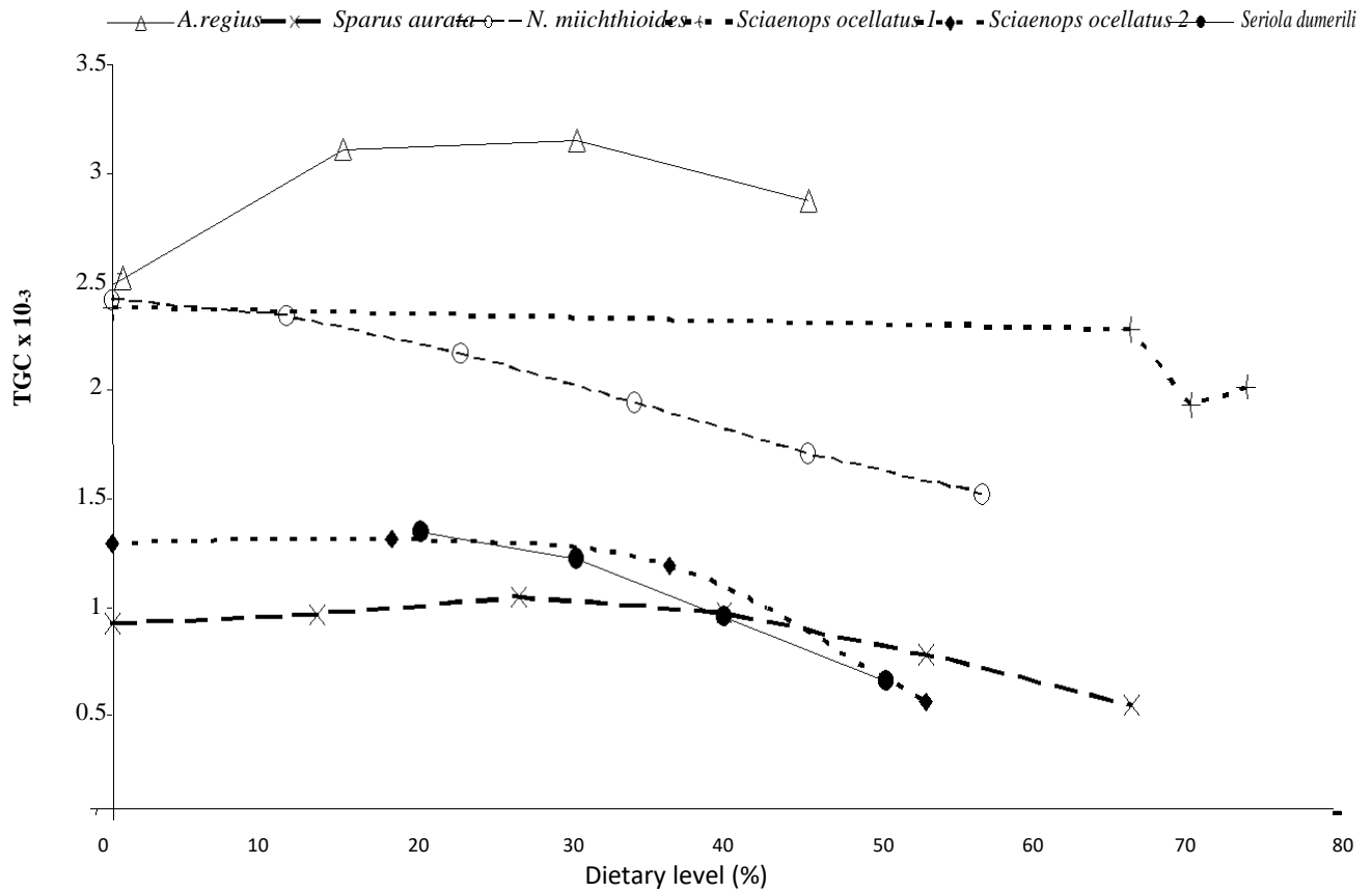
Figure 4. TGC of A. regius in the present trial, compared, Sparus aurata (Martínez-Llorens et al., 2009), N. miichthioides (Wang et al., 2006), Sciaenops ocellatus 1 (McGoogan and Gatlin III, 1997), Sciaenops ocellatus 2 (Reigh and Ellis, 1992) and Seriola dumerili (Tomás et al., 2005).
